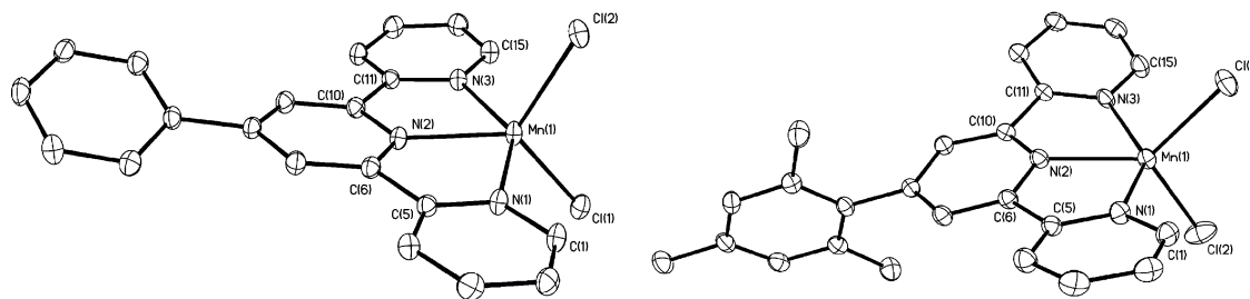
Figure 1. ORTEP diagrams of Mn II (Ph-terpy)Cl 2 ( 2e ) and Mn II (mesityl-terpy)Cl 2 ( 2g ), showing 30% probability thermal ellipsoids. Hydrogen atoms are omitted for clarity.
