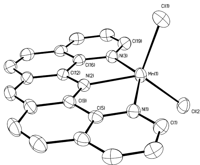
Figure 2. ORTEP diagram of Mn II (dpya)Cl 2 ( 2k ), showing 30% probability thermal ellipsoids. Hydrogen atoms are omitted for clarity. Selected bond distances (Å) and bond angles (deg):
