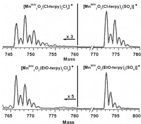
Figure 5. Selected ESI-MS data showing [\text{Mn}^{\text{III/IV}}_2(\mu\text{-O})_2(\text{L})_2\text{X}_2]^+ and [\text{Mn}^{\text{III/IV}}_2(\mu\text{-O})_2(\text{L})_2(\text{SO}_4)]^+ for L = Cl-terpy and EtO-terpy. Dotted lines show the simulated spectra in both cases. Corresponding peaks were also observed for L = terpy, Br-terpy, Ph-terpy, tolyl-terpy, mesityl-terpy, t Bu 3 -terpy, and py-phen.
