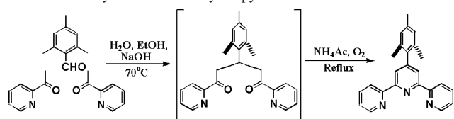
Scheme 1. Synthesis of Mesityl-terpy.
